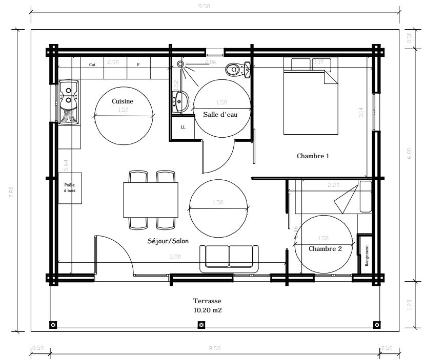
PLAN CHALETS B C D Ech:1/100e
