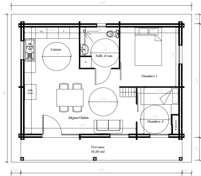
PLAN CHALET A Ech:1/100e
